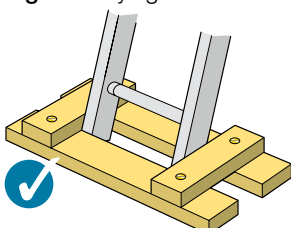
Figure 7 Securing at the base
